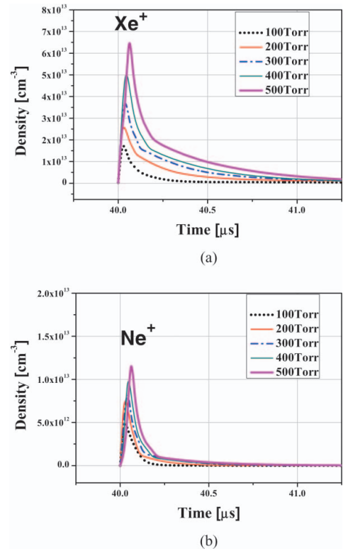
Figure 9. Comparison of (a) Xe and (b) Ne ions density based on simulated results during sustain discharge under various gas pressures.
